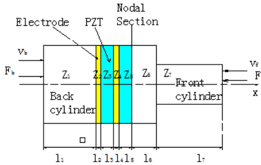
Fig. 3. Schematic of transducer
