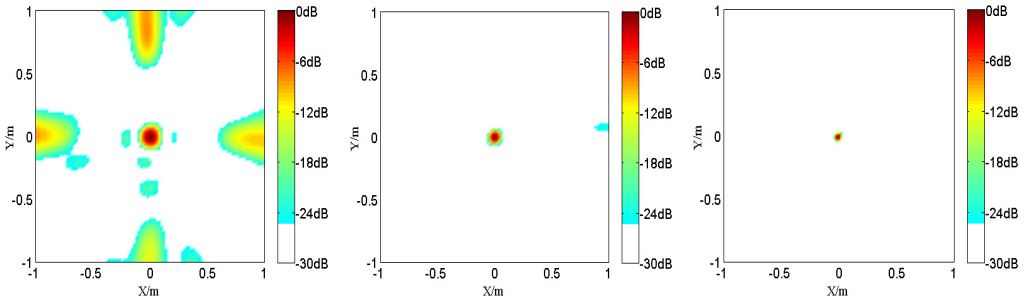
a) Improved FB with \nu = 1 b) Improved FB with \nu = 3 c) Improved FB with \nu = 10
