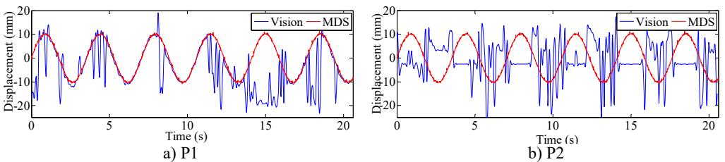
Fig. 4. Displacement time histories of case 2
