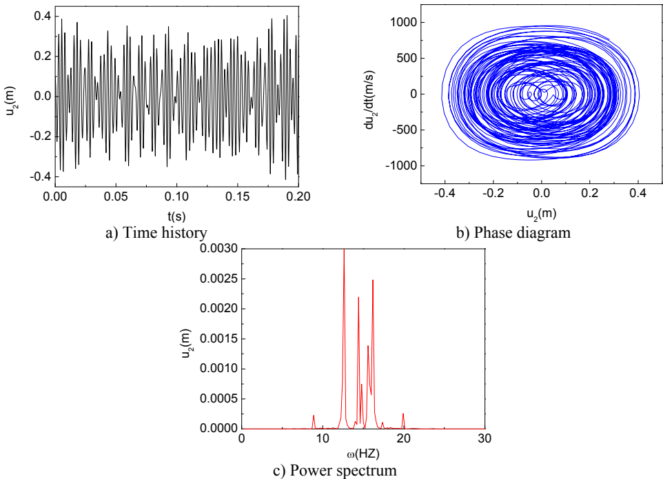
Fig. 13. Chaotic motion of the composite shaft ( \Omega = 2000 rad/s)
