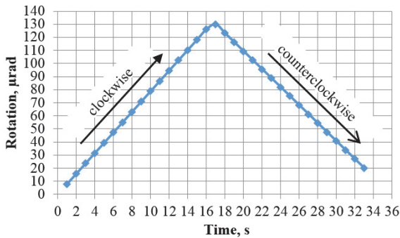
Fig. 5. Resolution of investigated piezotable – 7.9 µrad in clockwise direction and 6.9 µrad in counterclockwise direction
