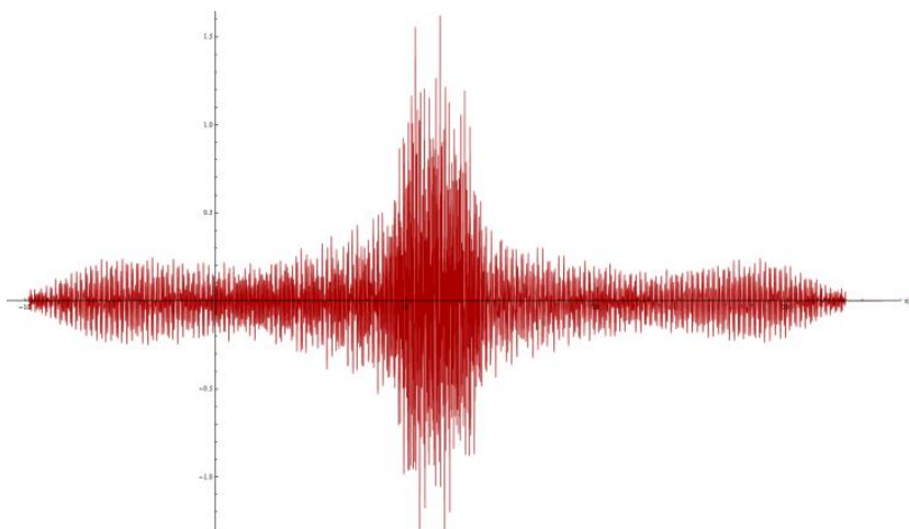
Fig. 22. Acceleration spectra modelled at the surface, \nu = 0.4
