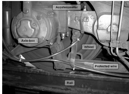
Fig. 1. Instrumented bogie
