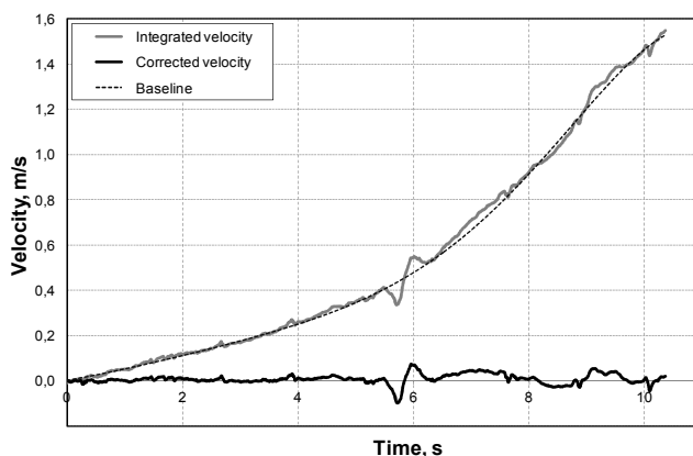
Fig. 5. Baseline correction in numerical integration
